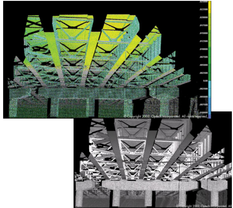
Images from top: False color deflection image in PolyWorks®, reference point cloud image and photograph of survey
